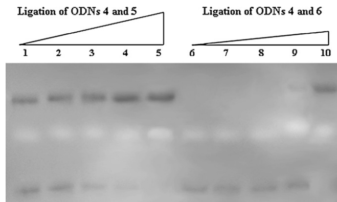
Figure 6. Denaturing gel electrophoresis assay of the time dependence of ligation at 4 °C (200 nM duplex concentration). (1) ODNs 5 , 4 , and template 3 : lane 1: 5 min; lane 2: 1.5 h; lane 3: 4 h; lane 4: 24 h; lane 5: 71 h; (2) ODNs 6 , 4 , and template 3 : lane 6: 5 min; Lane 7: 1.5; Lane 8: 4 h; Lane 9: 24 h; lane 10: 71 h (template bands not shown).
