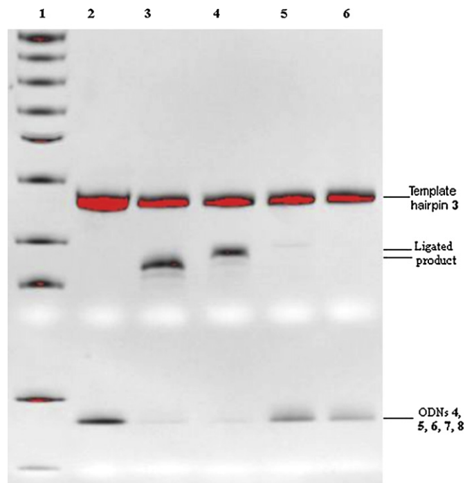
Figure 2. Denaturing gel electrophoresis assay of regioselectivity of templated ligation at room temperature (48 h, 200 nM duplex concentration). Lane 1: 10 base pairs marker; lane 2: ODNs 5, 4, and template 3 in absence of coupling reagent DMTMM as references; lane 3: ODNs 5, 4, and template 3; lane 4: ODNs 6, 4, and template 3; lane 5: ODNs 7, 4, and template 3; lane 6: ODNs 8, 4, and template 3.
