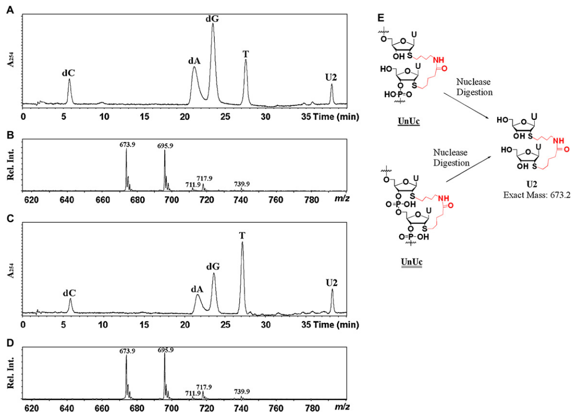
Figure 4. LC-MS analysis of nuclease full digestion products of ligation product 10 and control compound 9 . (A) UV chromatogram of 10 digestion products, (B) mass spectrum of fragment U2 from 10 digestion, (C) UV chromatogram of 9 digestion products, (D) mass spectrum of fragment U2 from 9 digestion, (E) structures of UnUc in 10 , UnUc in 9 and U2 . LC-MS eluent: A, water (0.1% formic acid); B, methanol (0.1% formic acid). Gradient: 0 min, 95% A; 2 min, 95% A; 5 min, 65% A; 40 min, 15% A; 45 min, 0% A.
