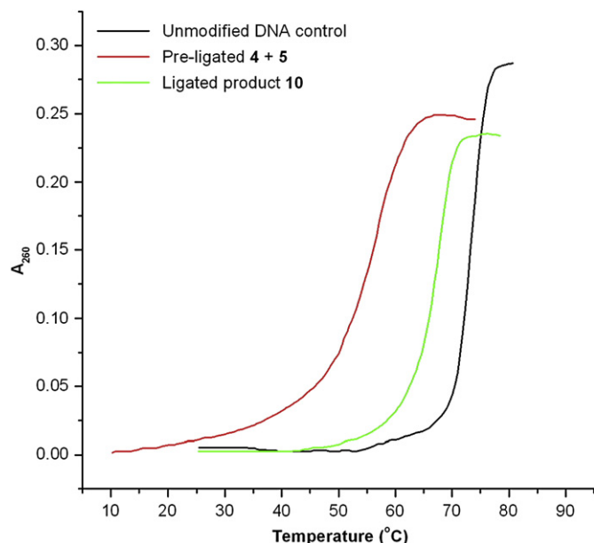
Figure 5. Melting curves of DNA control, pre-ligated 4/5 , and ligated strand 10 with complementary natural DNA. A_{260} = [A_{260}(T_0) - A_{260}(T)] / A_{260}(T_0) ( A_{260}(T_0) is the absorbance at 25 °C for DNA control and ligated strand 10 , the absorbance at 10 °C for pre-ligated 4/5 ). Unmodified DNA control: 5'-AACACGGACATAGTTCCTCGTGTGTTGGAC-3'. Complementary DNA: 5'-GTCCACAACACGAGGAACATATGTCCTGTT-3'.
