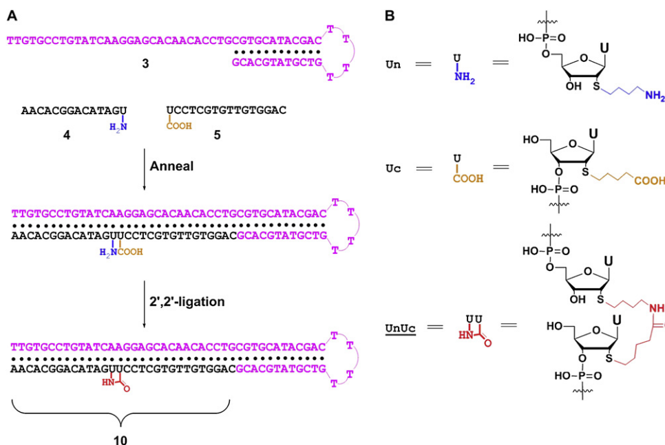
Figure 1. Schematic depiction of the template-mediated 2',2'-ligation of two ODNs. (A) Two end-modified ODNs are aligned together by forming duplex with a DNA hairpin template and then proximal amine and carboxylate are connected using chemical ligation. (B) Symbols and chemical structures representing ligation units.
