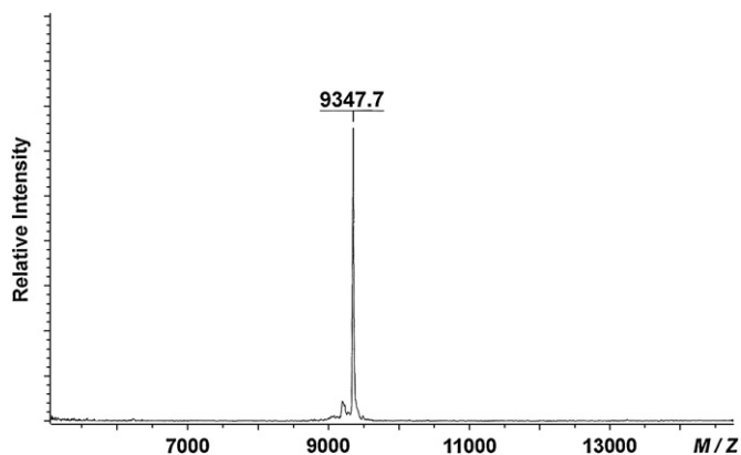
Figure 3. MALDI-TOF MS of the ligated product 10 from templated ligation of ODNs 4 and 5 .
